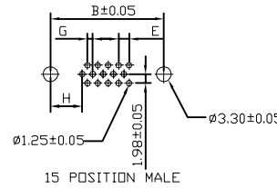
15 POSITION MALE
