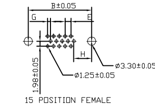
15 POSITION FEMALE
