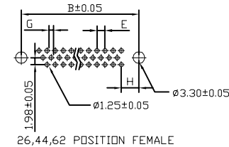
26,44,62 POSITION FEMALE
