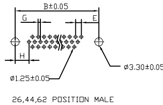
26,44,62 POSITION MALE
